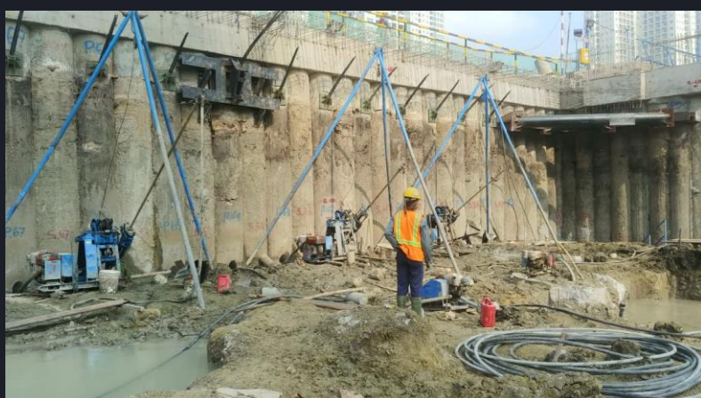
ENSURING THE STRENGTH OF GROUND ANCHOR
