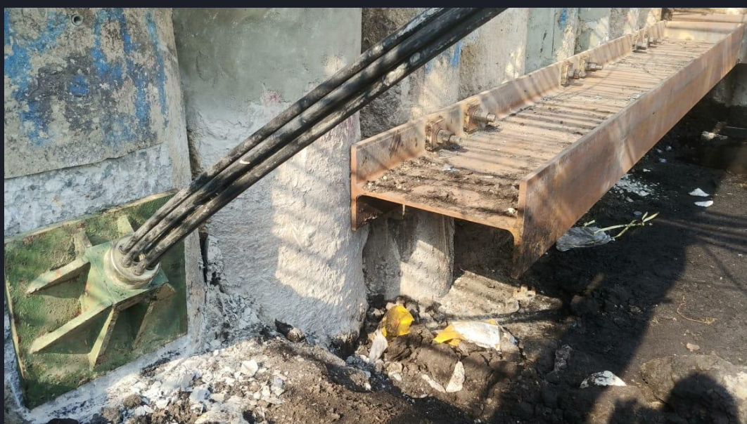
STRUTTING SYSTEM FOR DEEP BASEMENT: SAFETY FIRST
