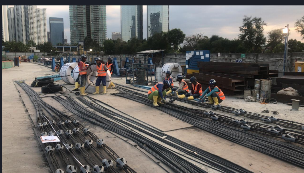
PREPARING TENDON BAR FOR GROUND ANCHOR INSTALLATION
